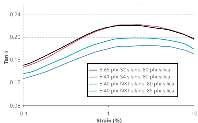
Figure 6: Tan \delta max Values, 10.0 Hz, @ 55 °C
