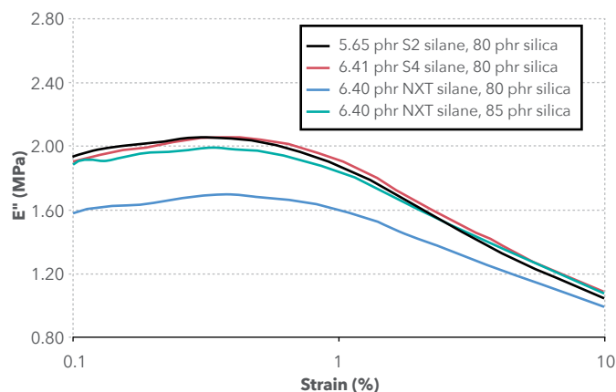
Figure 7: E'' Values, 10.0 Hz, @ 55 °C
